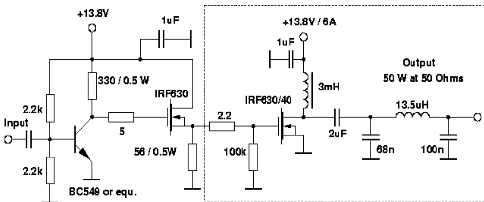
Driver and Power Amplifier, 137 kHz
